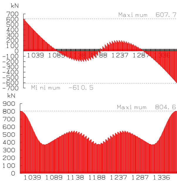
Fig. 15. Comparison of internal shear force due to lateral wind with static (top) and dynamic (bottom) contribution.
