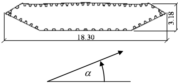
Fig. 1. Deck cross section of Hardanger bridge with definition of wind incident angle
