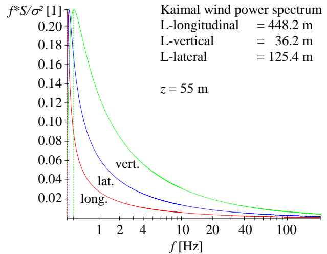
Fig. 12. Power spectra of longitudinal, vertical and lateral fluctuating wind components.
