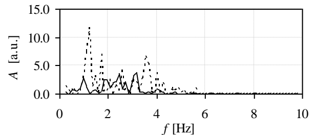
Fig. 6. Moment power spectrum with (solid) and without (dashed) guiding vanes.
