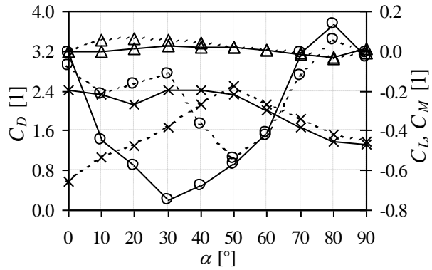
Fig. 10. Steady state coefficients C_D (x), C_L (O) and C_M ( \Delta ) for left (solid) and right (dashed) pylon leg.
