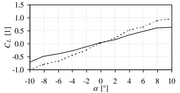
Fig. 4. Lift coefficient for deck with (solid) and without (dashed) wind guiding vanes.
