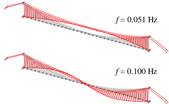
Fig. 14. First two eigenmodes of Hardanger bridge deck.
