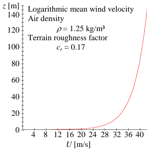
Fig. 11. Mean wind profile.
