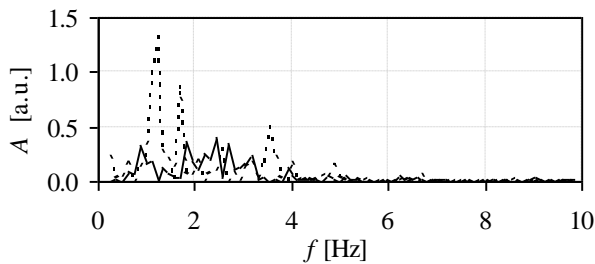
Fig. 5. Lift force power spectrum with (solid) and without (dashed) guiding vanes.
