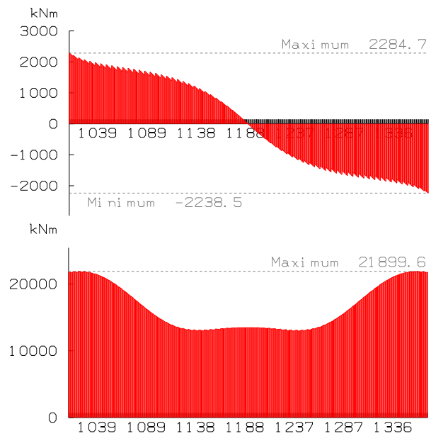
Fig. 16. Comparison of longitudinal twisting moment due to lateral wind with static (top) and dynamic (bottom) contribution.
