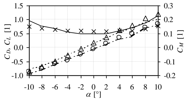
Fig. 2. Steady state coefficients of Hardanger bridge deck: C_D (x), C_L (O) and C_M (Δ)
