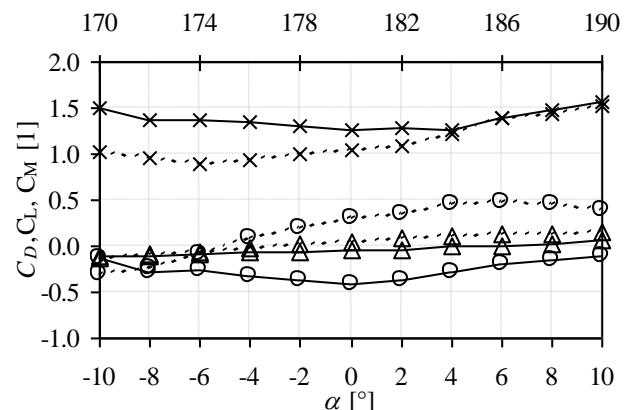
Fig. 8. Steady state coefficients C_D (x), C_L (O) and C_M ( \Delta ) for traffic on both lanes for wind from left (solid) and right (dashed).
