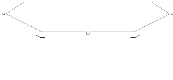
Fig. 3. Cross section with wind guiding vanes and spoiler for Hardanger bridge.
