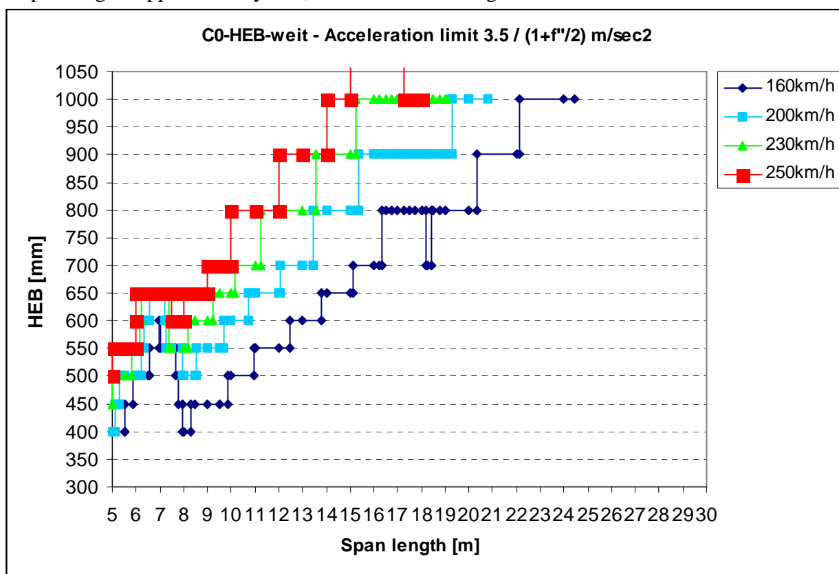
Fig. 8. Required plate depth and steel sections as a function of the span length (limit 3.5 \text{ m/s}^2 )
