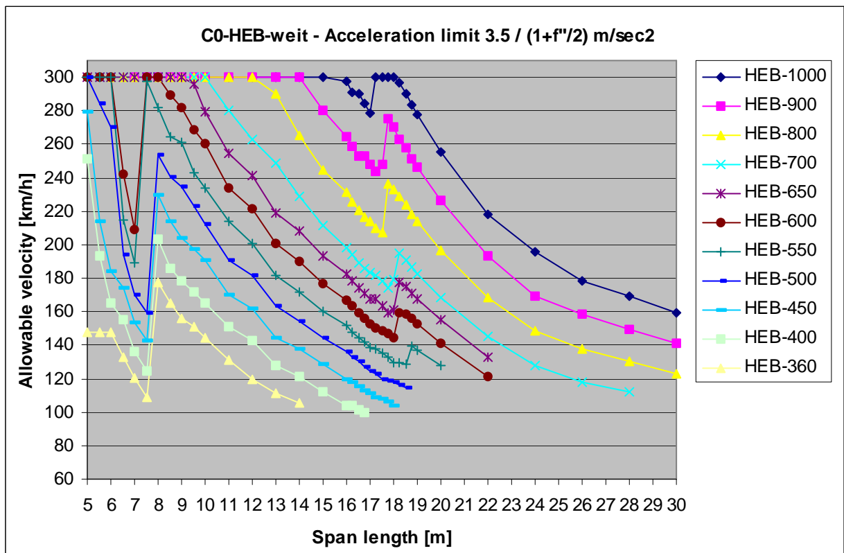
Fig. 7. Allowable travel speeds for new structures (limit 3.5 \text{ m/s}^2 )
