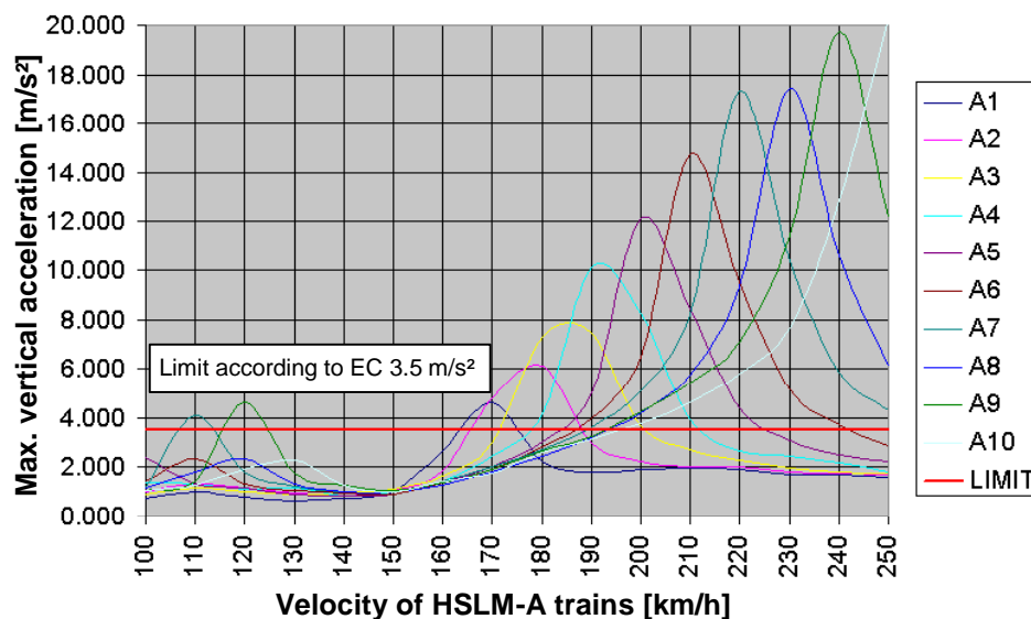
Fig. 3. Maximum vertical acceleration for different trains
