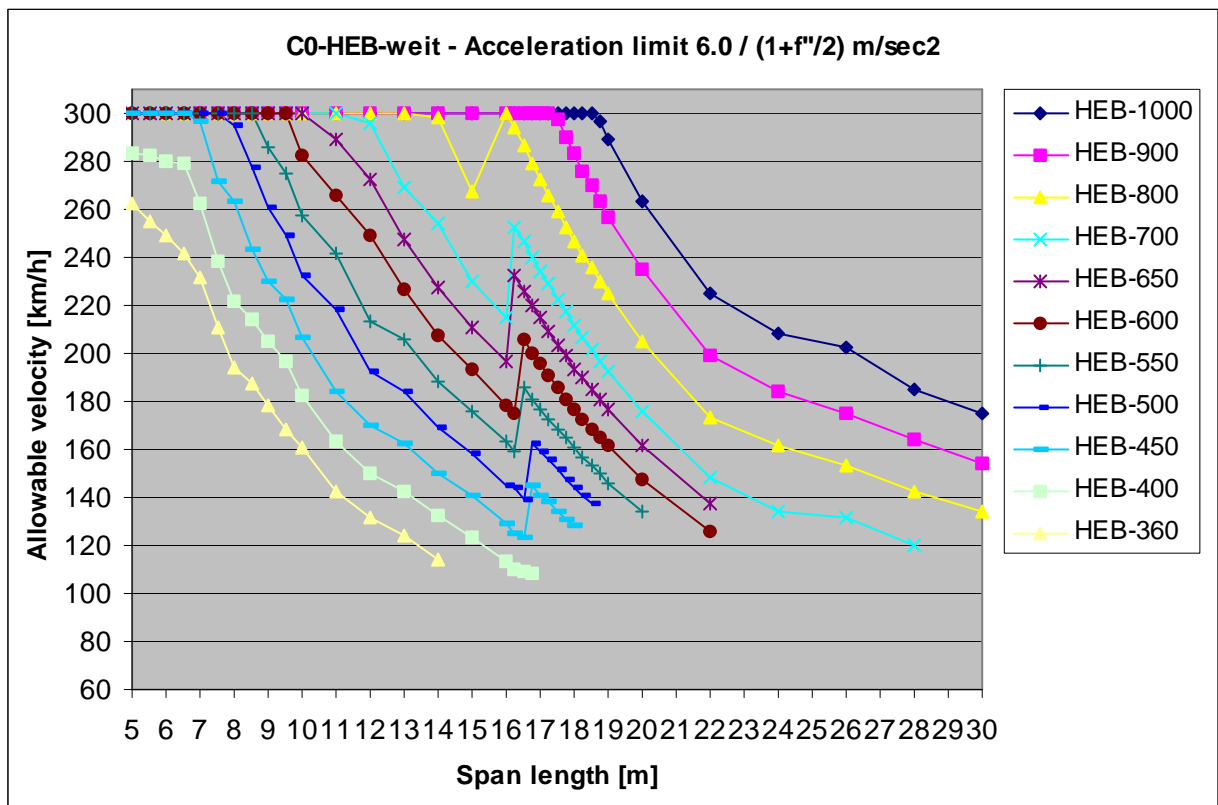
Fig. 6. Allowable travel speeds for existing structures (limit 6.0 \text{ m/s}^2 )
